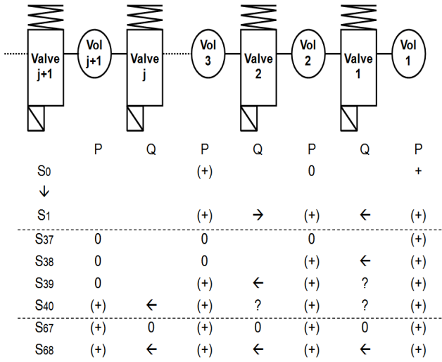
Figure 4 - Volume-Valve sequence
