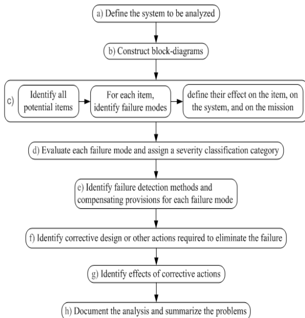
Figure 1 - FMEA process
