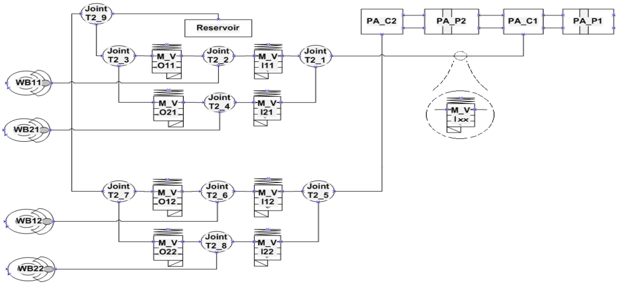
Figure 2 - Braking system. Pressure is generated by two pistons, PA_P1,2, in two chambers, PA_CA1,2, and reaches the wheel brakes, WB ij , via open inlet valves, M_V Iij , while outflow is blocked by closed outlet valves, M_V Oij . The impact of inserting another valve, M_V Ixx , is discussed in section 5.3
