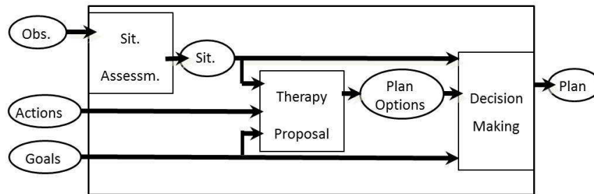
Fig. 1. General Architecture of a DSS
