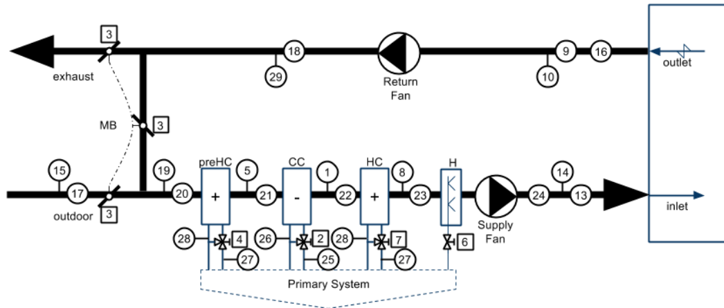
Figure 1 Air Handling Unit schematic
